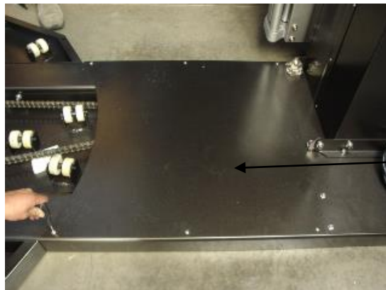
Remove top panel to expose chain
